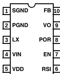
EL7535 (10 LD MSOP) TOP VIEW
