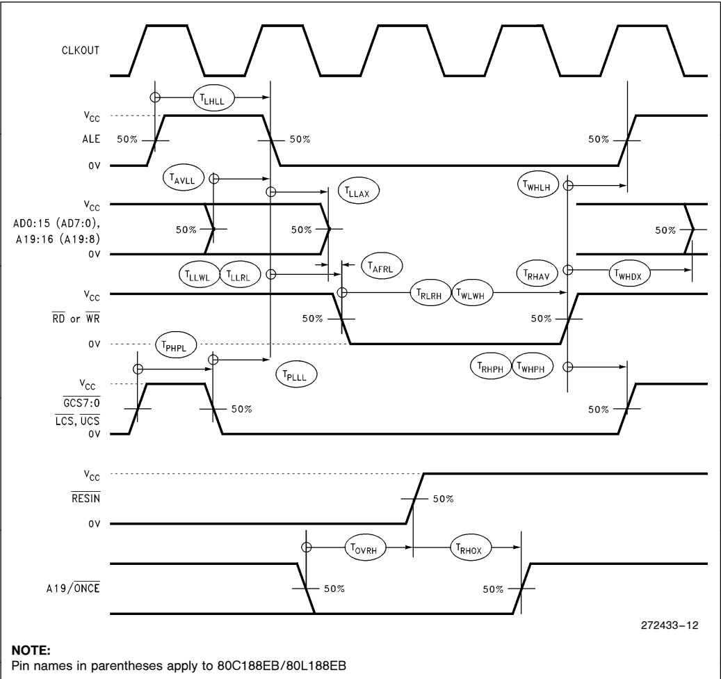
Figure 11. Relative Signal Waveform
