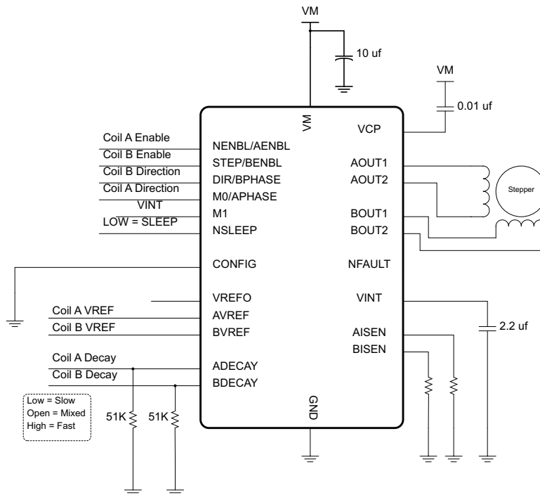
Figure 11. High-Resolution Microstepping
