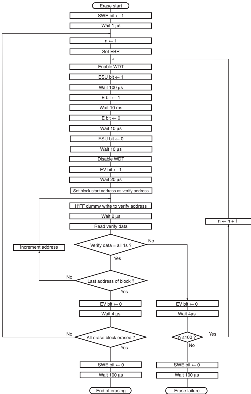
Figure 6.11 Erase/Eraser-Verify Flowchart
