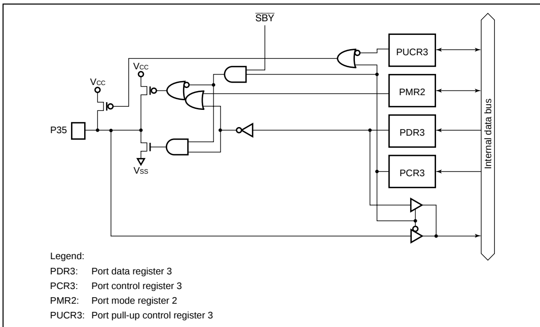
Figure B.1(b) Port 3 Block Diagram (Pin P35)
