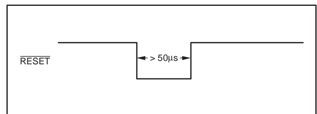
Figure 9. Reset Timing
