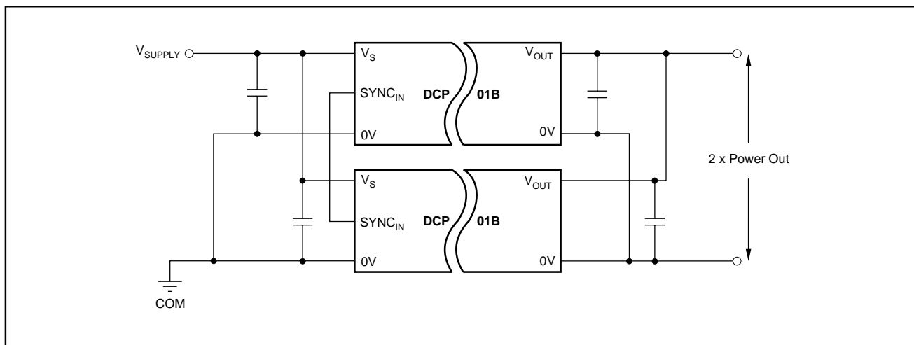
FIGURE 3. Connecting Multiple DCP01Bs in Parallel.
