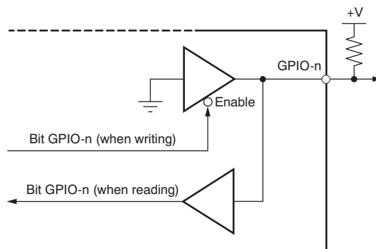
Figure 99. GPIO-n Pin
