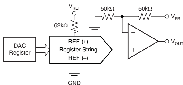
Figure 46. DAC8551 Architecture
