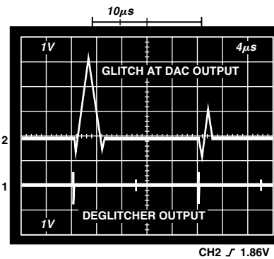
Figure 33. Glitch and Deglitched Results
