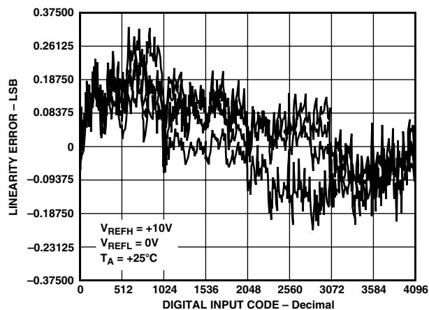
Figure 15. Channel-to-Channel Matching ( V_{SUPPLY} = \pm 15 V )
