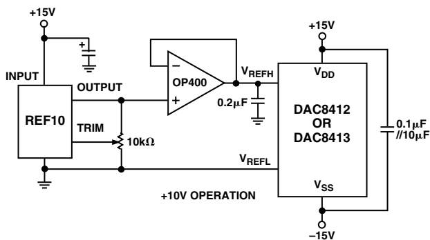
Figure 36. Unipolar +10 V Operation
