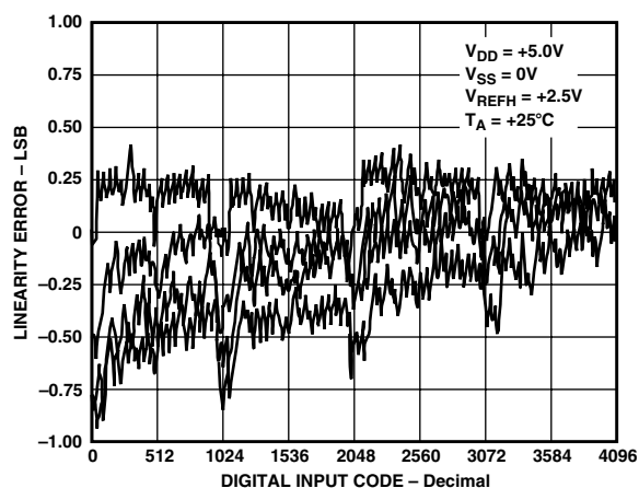
Figure 16. Channel-to-Channel Matching ( V_{SUPPLY} = +5 V/GND )
