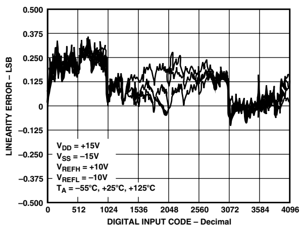
Figure 18. INL vs. Code
