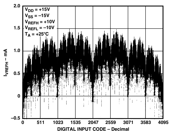
Figure 19. I_{VREFH} vs. Code
