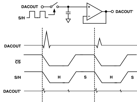
Figure 34. Deglitcher Circuit
