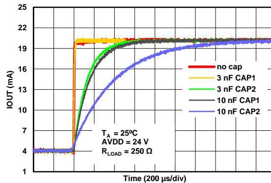
Figure 88. IOOUT vs Time for Different Capacitor Values on CAP1 and CAP2
