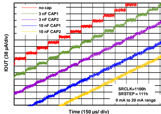
Figure 86. IOOUT vs Time With Digital Slew Rate Control
