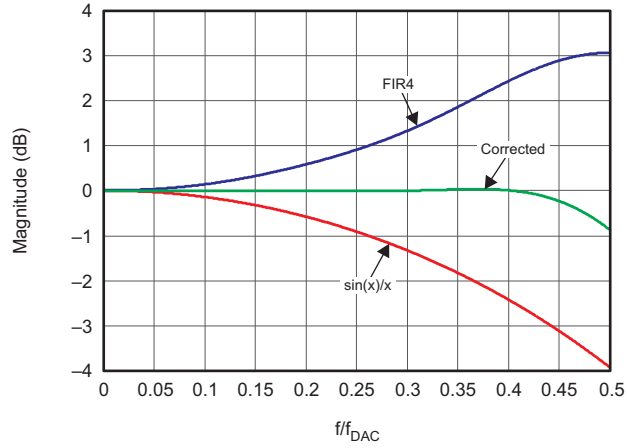
Figure 16. Magnitude Spectrum for Inverse Sinc Filter G056
