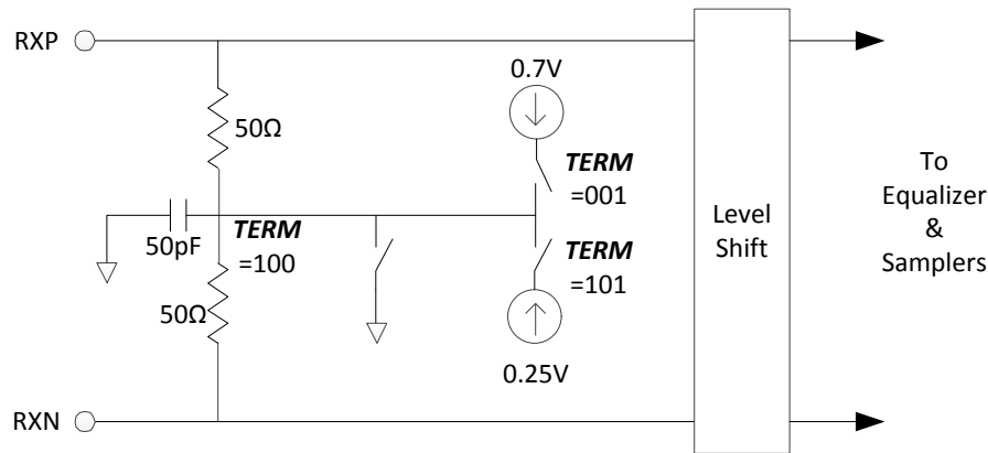
Figure 1. Serial Lane Input Termination
