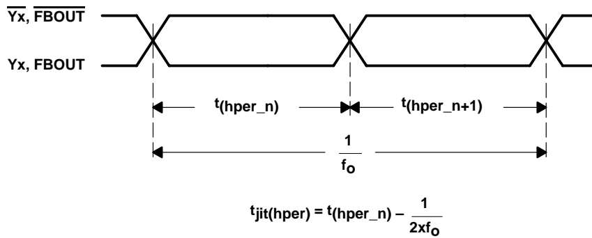
Figure 6. Half-Period Jitter
