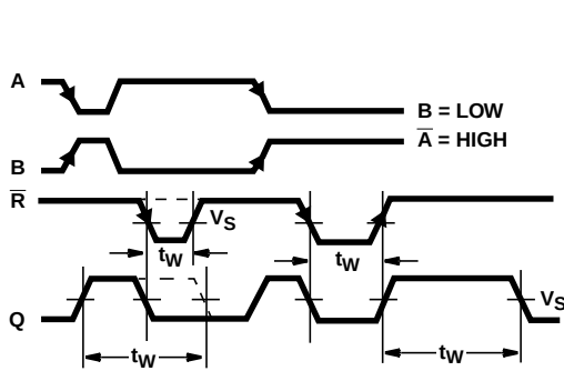
FIGURE 1. OUTPUT PULSE CONTROL USING RESET INPUT (R) PULSE FOR 123
