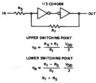
Fig. 22 - Input pulse shaping circuit (Schmitt trigger).
