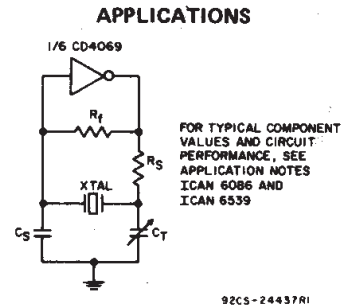
Fig. 19 - Typical crystal oscillator circuit.
