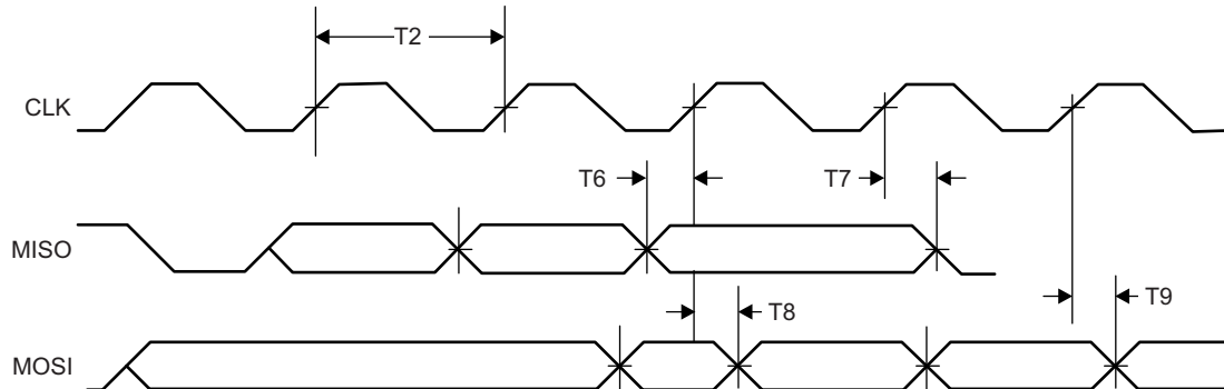
Figure 5-8. SPI Master Timing Diagram
