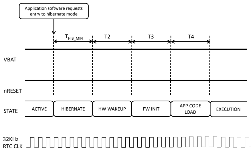
Figure 5-7. Wake Up From Hibernate Timing Diagram
