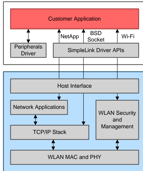
Figure 1-3. CC3220x Embedded Software Overview
