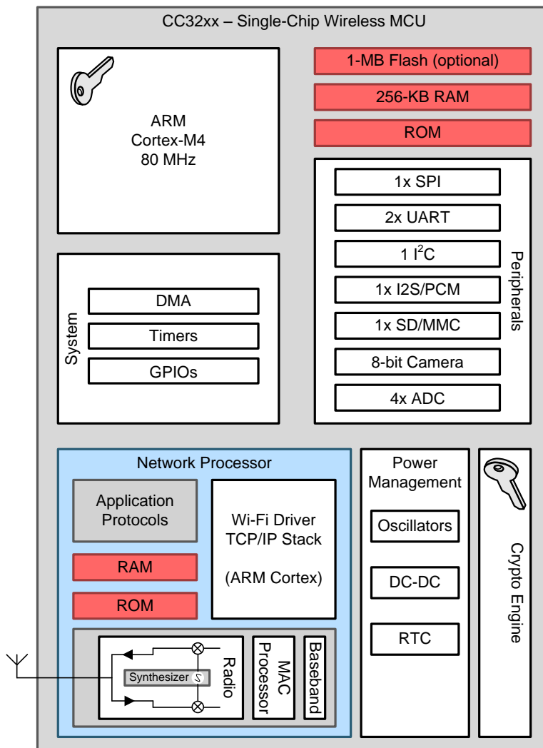
Figure 1-2. CC3220x Hardware Overview
