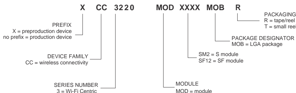
Figure 9-1. CC3220MODx Module Nomenclature
