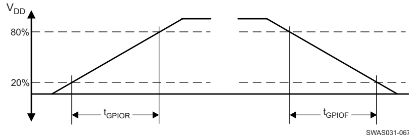
Figure 5-12. GPIO Timing Diagram
