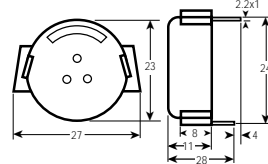
BRP2711P-30 Series
