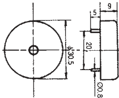
BRP3009P-30 Series
