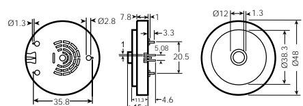
BRP4815-30-TR Series
