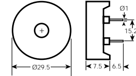
BRP3008-P-30-LF Series
