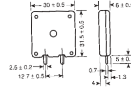
BSP3206 Series
