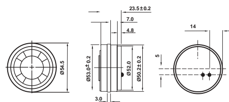
BPS5524SP-150 Series
