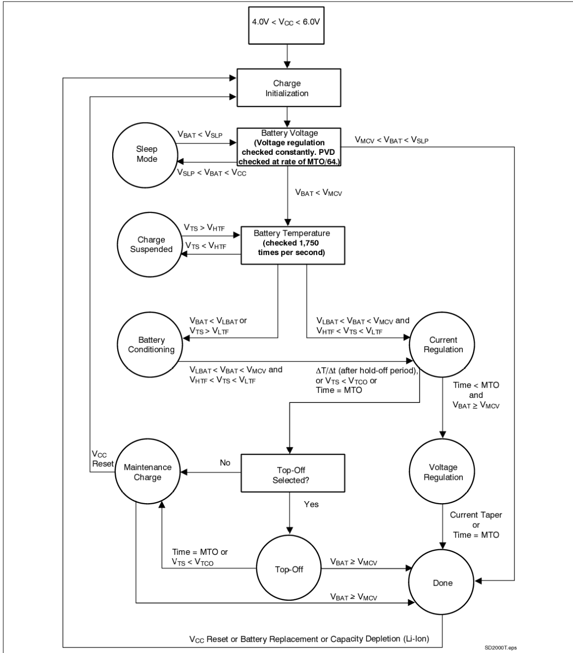
Figure 2. State Diagram
