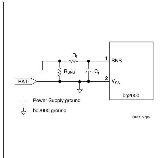
Figure 9. Current-Sensing Circuit
