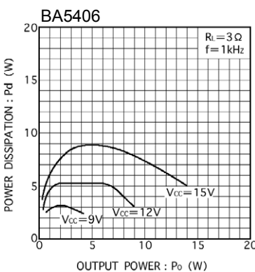
Fig.17 Power dissipation vs Output power(3)
