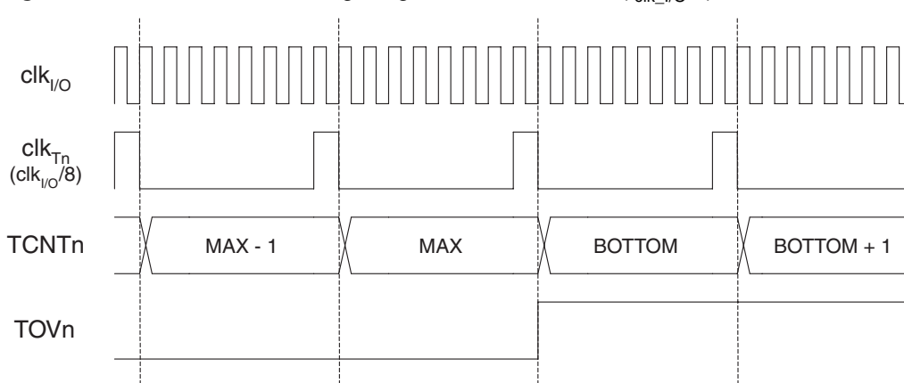
Figure 61. Timer/Counter Timing Diagram, with Prescaler ( f_{\text{clk}_{I/O}}/8 )
