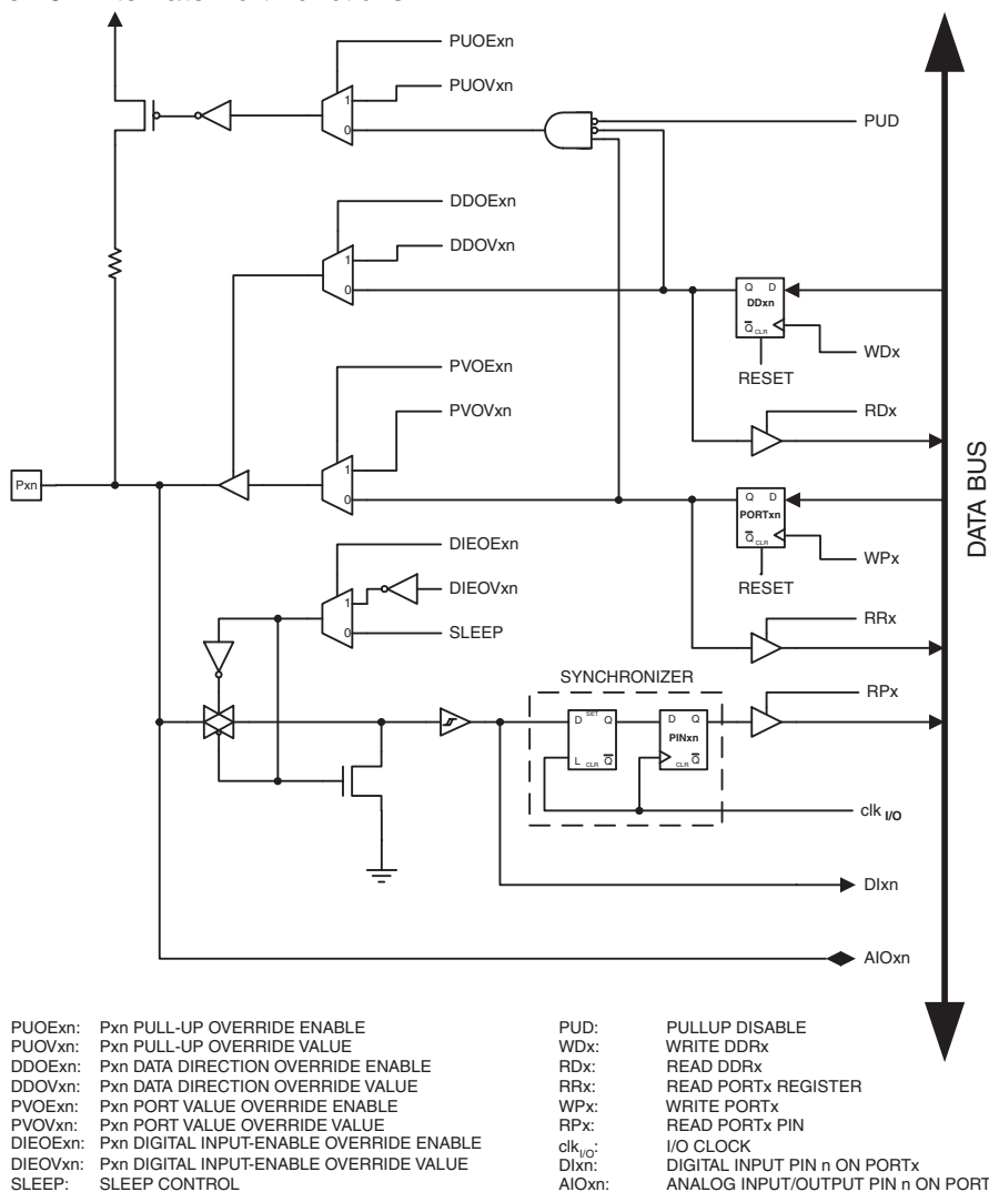
Figure 26. Alternate Port Functions (1)
