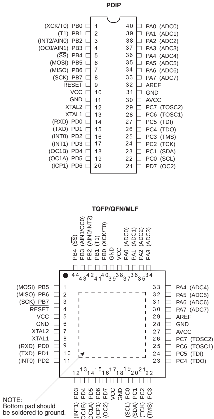
Figure 1. Pinout ATmega16
