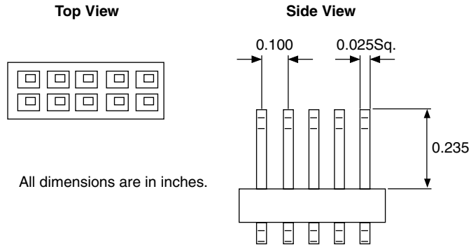
Figure 4-1. 10-pin Male Header Dimensions
