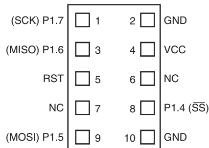
Figure 3-1. AT89ISP Cable 10-pin Male Header Pinout
