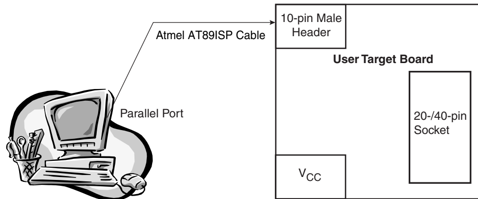
Figure 5-2. AT89ISP Target Board Sample Connection
