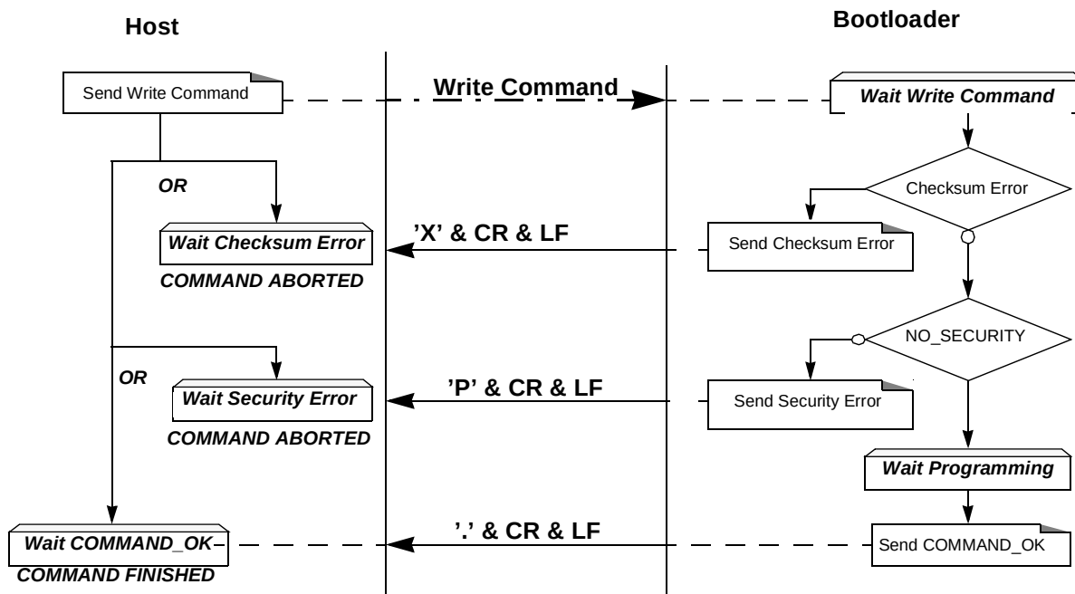
Figure 48. Write/Program Flow
