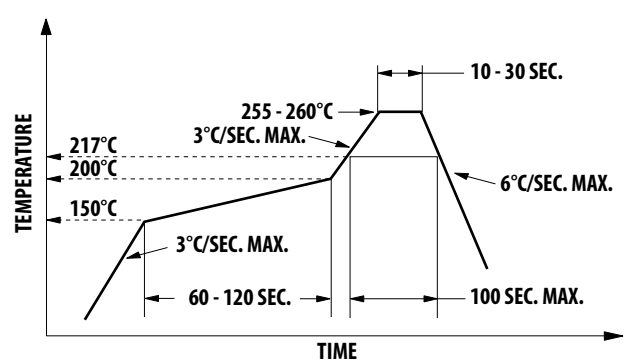
Figure 11 Recommended Pb-Free Soldering Profile
