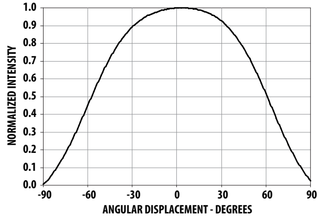
Figure 9 Radiation Pattern
