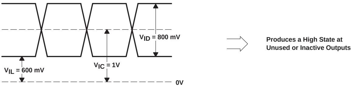
Figure 6. Waveform Three
