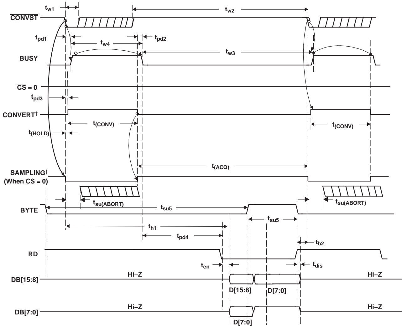
Figure 34. Timing for Conversion and Acquisition Cycles With \overline{CS} Tied to BGDND, \overline{RD} Toggling
