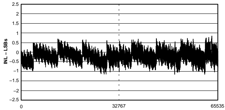
Figure 50. Typical INL
