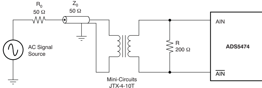
Figure 32. Converting a Single-Ended Input to a Differential Signal Using an RF Transformer
