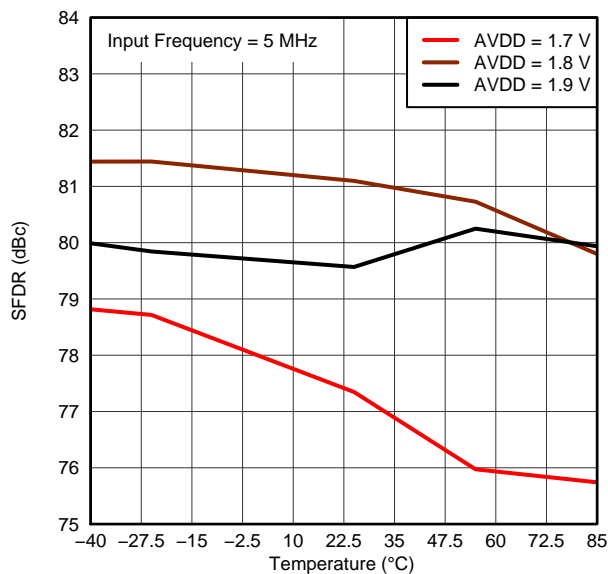
Figure 52. SPURIOUS-FREE DYNAMIC RANGE vs AVDD AND TEMPERATURE
