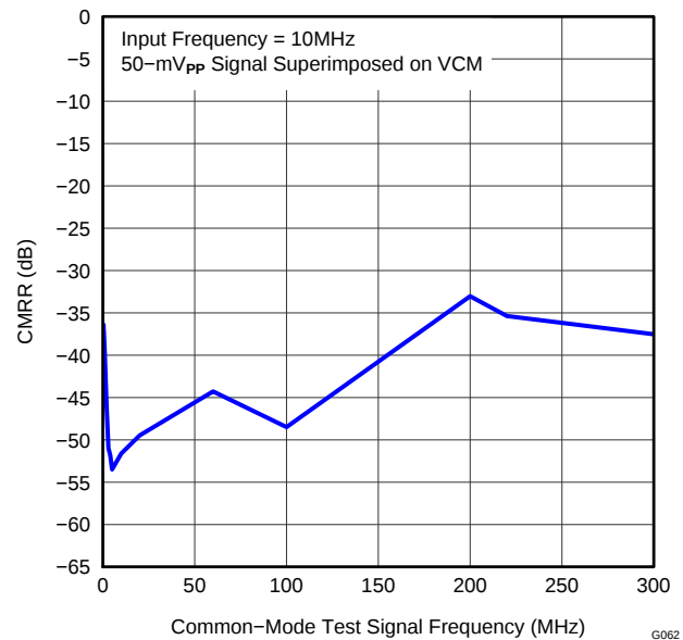
Figure 72. CMRR vs TEST SIGNAL FREQUENCY
