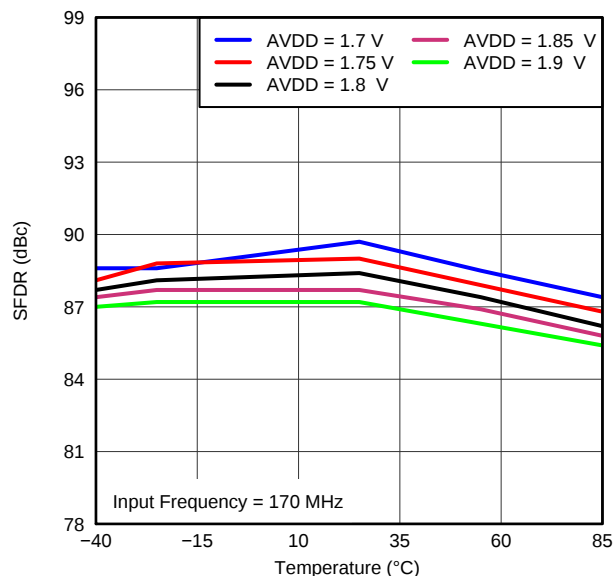
Figure 31. SFDR vs AVDD SUPPLY AND TEMPERATURE (170 MHz)
