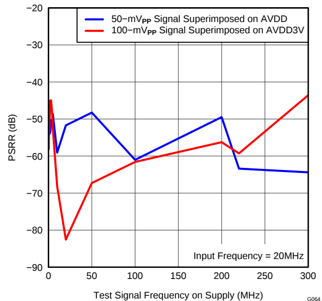
Figure 74. PSRR vs TEST SIGNAL FREQUENCY
