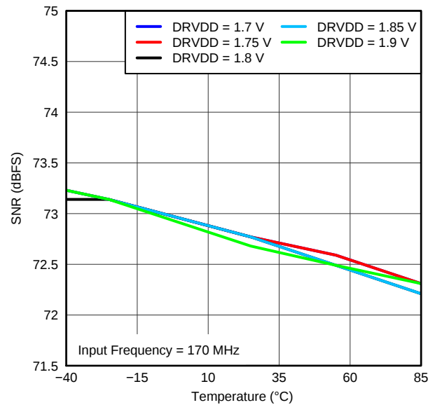
Figure 66. SNR vs DRVDD SUPPLY AND TEMPERATURE (170 MHz)
