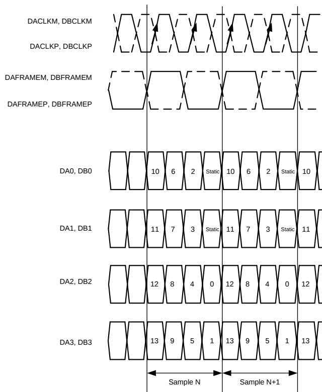
Figure 102. QDR LVDS Interface Timing: ADS42LB49
