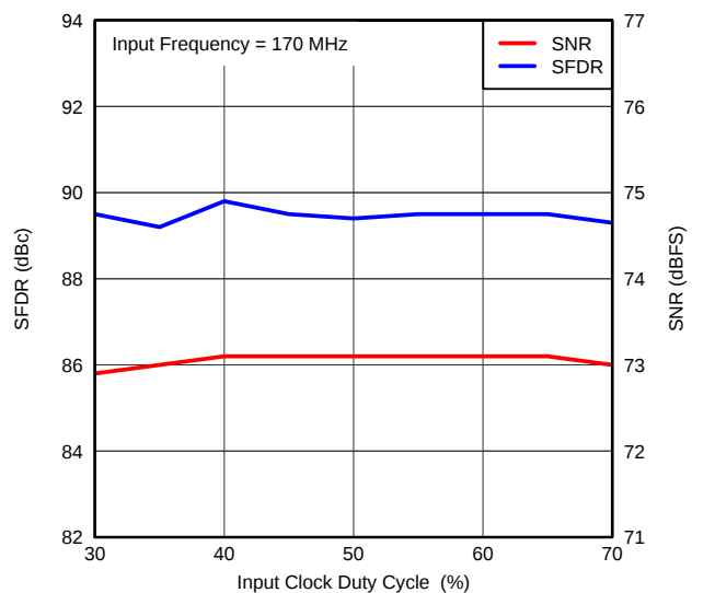
Figure 40. PERFORMANCE vs CLOCK DUTY CYCLE (170 MHz)
