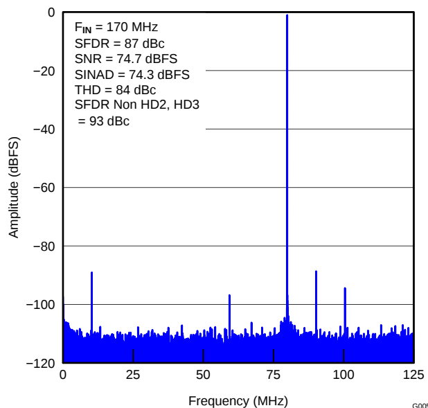
Figure 15. FFT FOR 170-MHz INPUT SIGNAL (2.5- V_{\text{PP}} Full-Scale)
