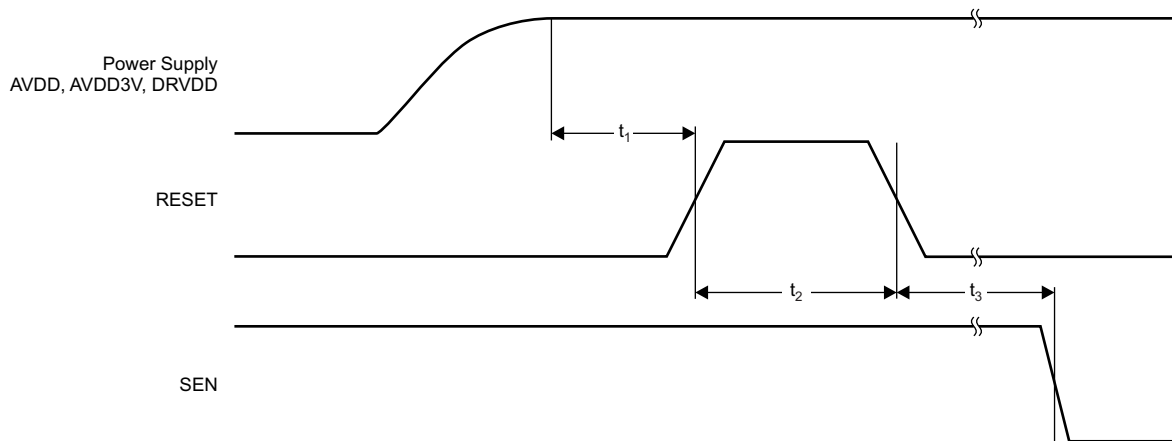
Figure 82. Reset Timing Diagram
