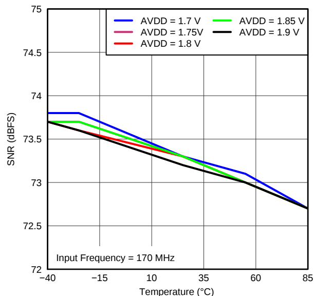
Figure 32. SNR vs AVDD SUPPLY AND TEMPERATURE (170 MHz)
