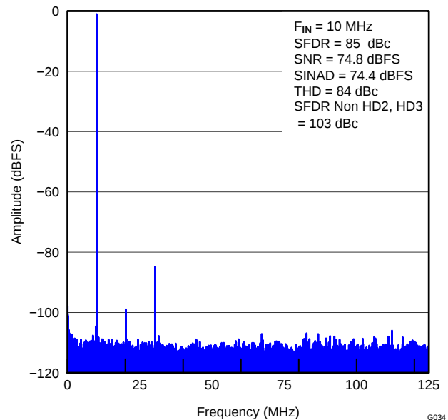
Figure 44. FFT FOR 10-MHz INPUT SIGNAL (2.5- V_{\text{PP}} Full-Scale)
