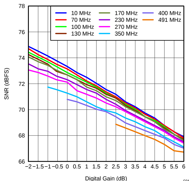
Figure 56. SNR vs DIGITAL GAIN
