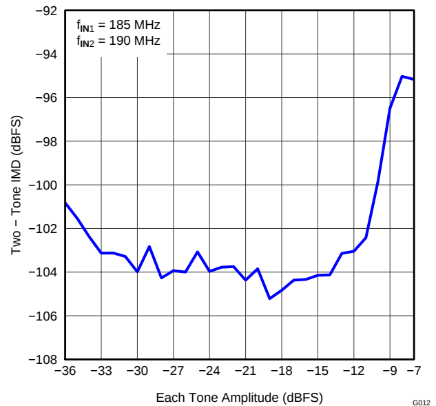
Figure 22. IMD3 vs INPUT AMPLITUDE (185 MHz and 190 MHz)
