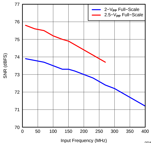
Figure 24. SNR vs INPUT FREQUENCY
