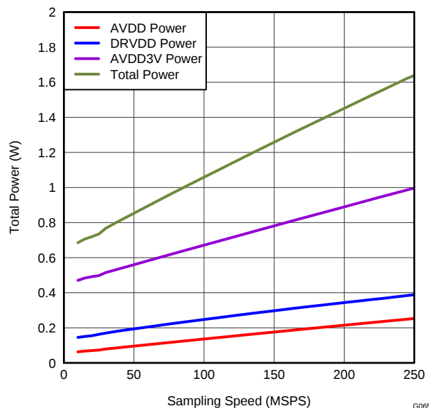
Figure 75. TOTAL POWER vs SAMPLING FREQUENCY
