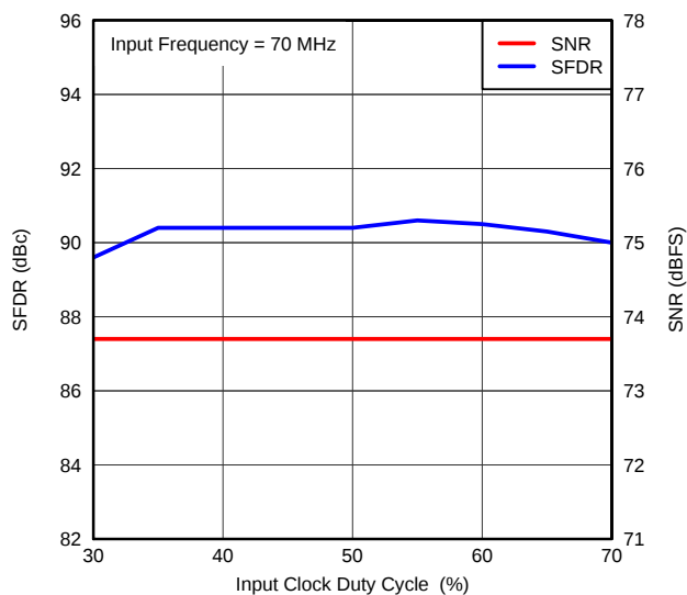
Figure 39. PERFORMANCE vs CLOCK DUTY CYCLE (70 MHz)
