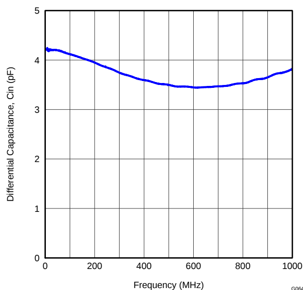
Figure 87. ADC Analog Input Capacitance ( C_{IN} ) Across Frequency
