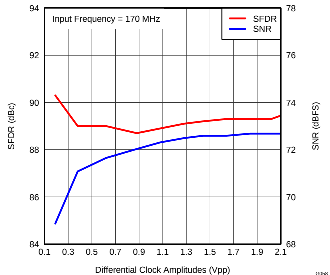
Figure 68. PERFORMANCE vs CLOCK AMPLITUDE (170 MHz)
