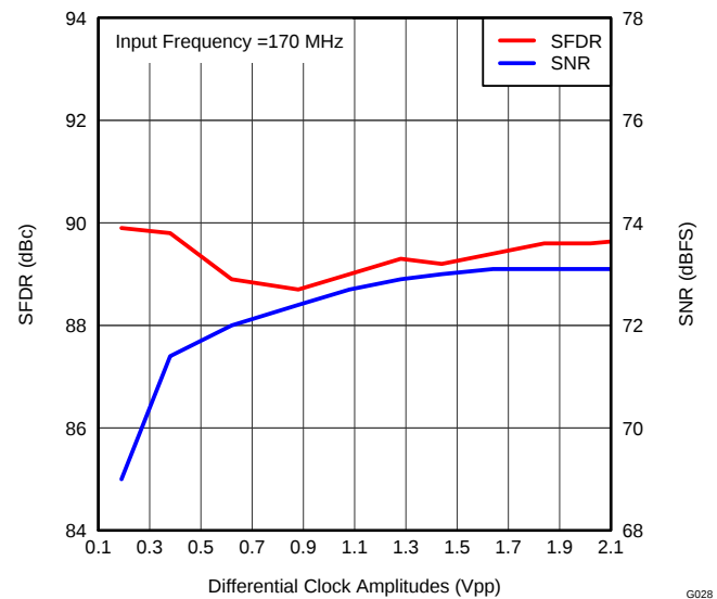
Figure 38. PERFORMANCE vs CLOCK AMPLITUDE (170 MHz)
