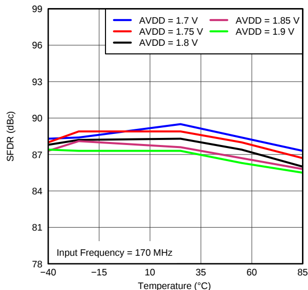
Figure 61. SFDR vs AVDD SUPPLY AND TEMPERATURE (170 MHz)
