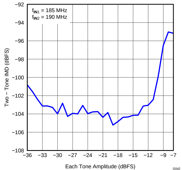
Figure 52. IMD3 vs INPUT AMPLITUDE (185 MHz and 190 MHz)
