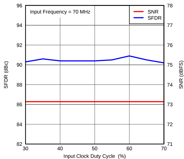
Figure 69. PERFORMANCE vs CLOCK DUTY CYCLE (70 MHz)
