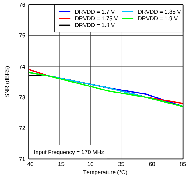
Figure 36. SNR vs DRVDD SUPPLY AND TEMPERATURE (170 MHz)
