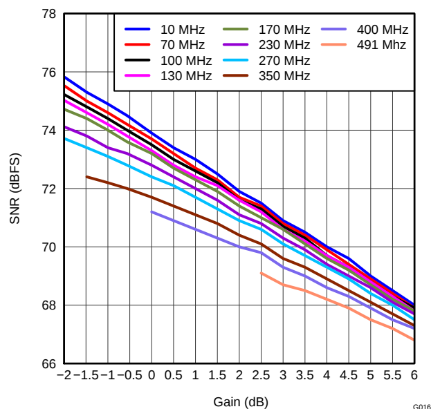
Figure 26. SNR vs DIGITAL GAIN
