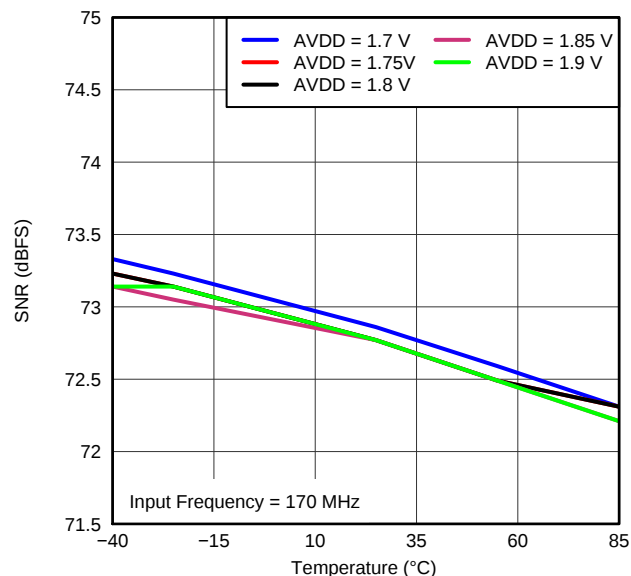
Figure 62. SNR vs AVDD SUPPLY AND TEMPERATURE (170 MHz)
