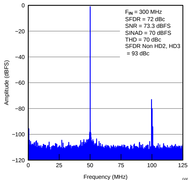
Figure 16. FFT FOR 300-MHz INPUT SIGNAL (2.5- V_{\text{PP}} Full-Scale)
