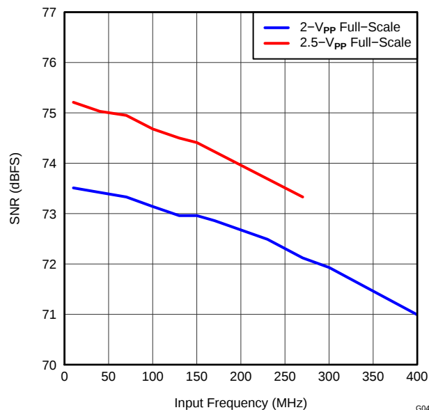
Figure 54. SNR vs INPUT FREQUENCY
