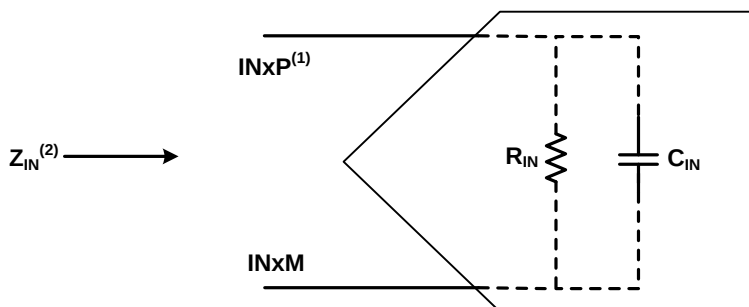
Figure 85. ADC Equivalent Input Impedance
