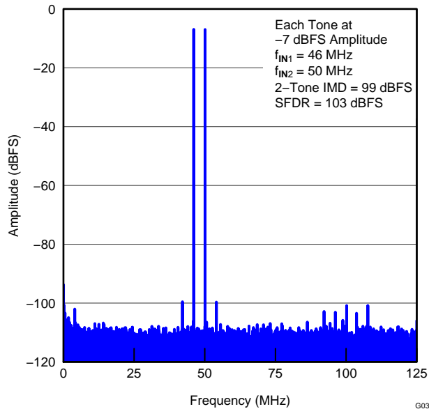
Figure 47. FFT FOR TWO-TONE INPUT SIGNAL (At -7 dBFS, 46 MHz and 50 MHz)
