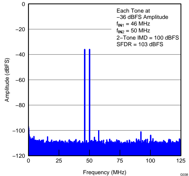
Figure 48. FFT FOR TWO-TONE INPUT SIGNAL (At -36 dBFS, 46 MHz and 50 MHz)
