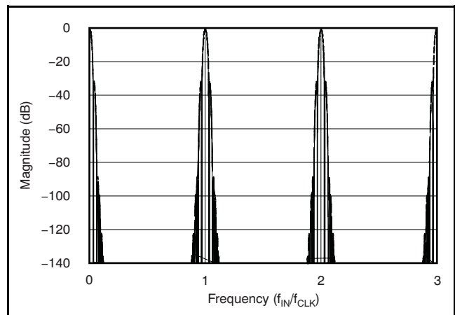
Figure 30. Extended Frequency Response of Low-Latency Path
