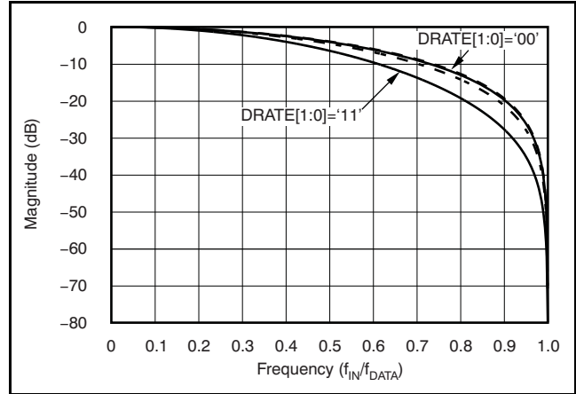
Figure 29. Frequency Response of Low-Latency Filter in Fast-Response Configuration
