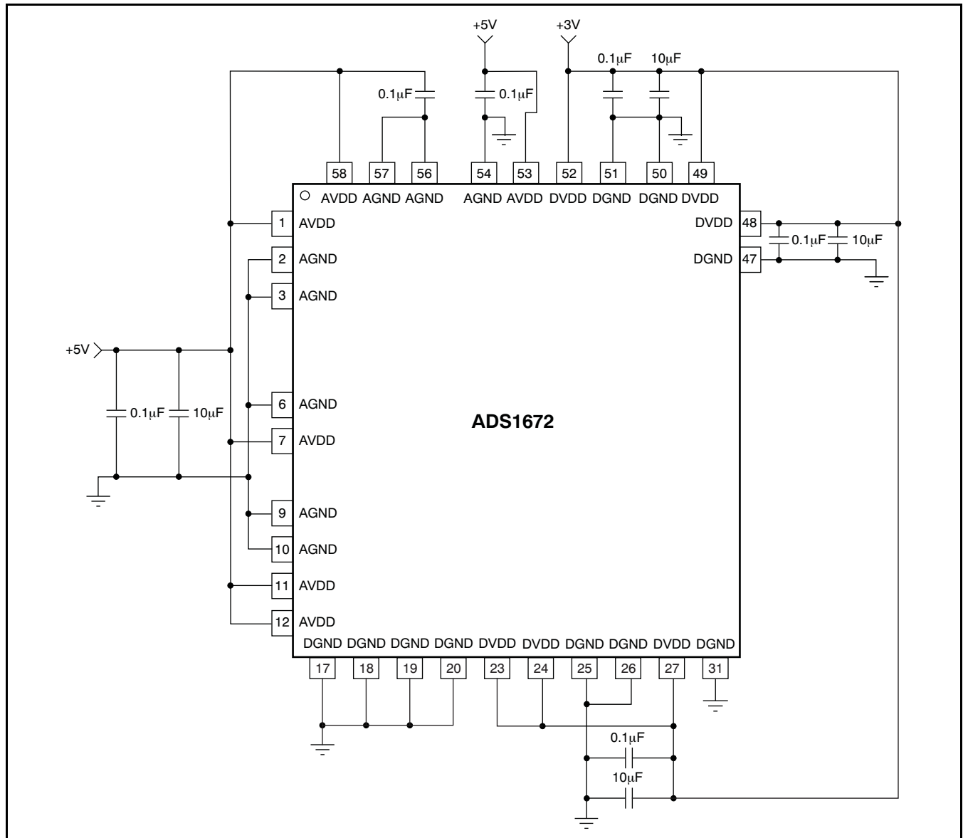
Figure 40. Power-Supply Decoupling
