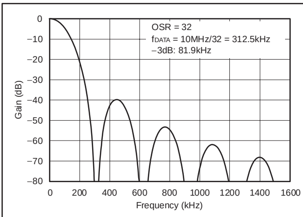
Figure 7. Frequency Response of Sinc 3 Filter
