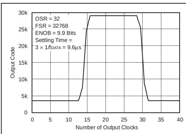
Figure 8. Pulse Response of Sinc 3 Filter ( f_{MOD} = 10\text{MHz} )
