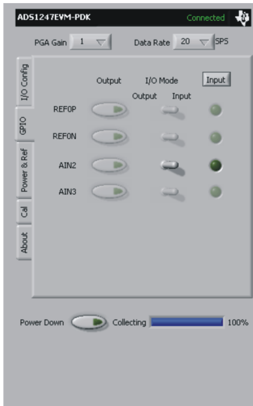
Figure 18. GPIO Tab
