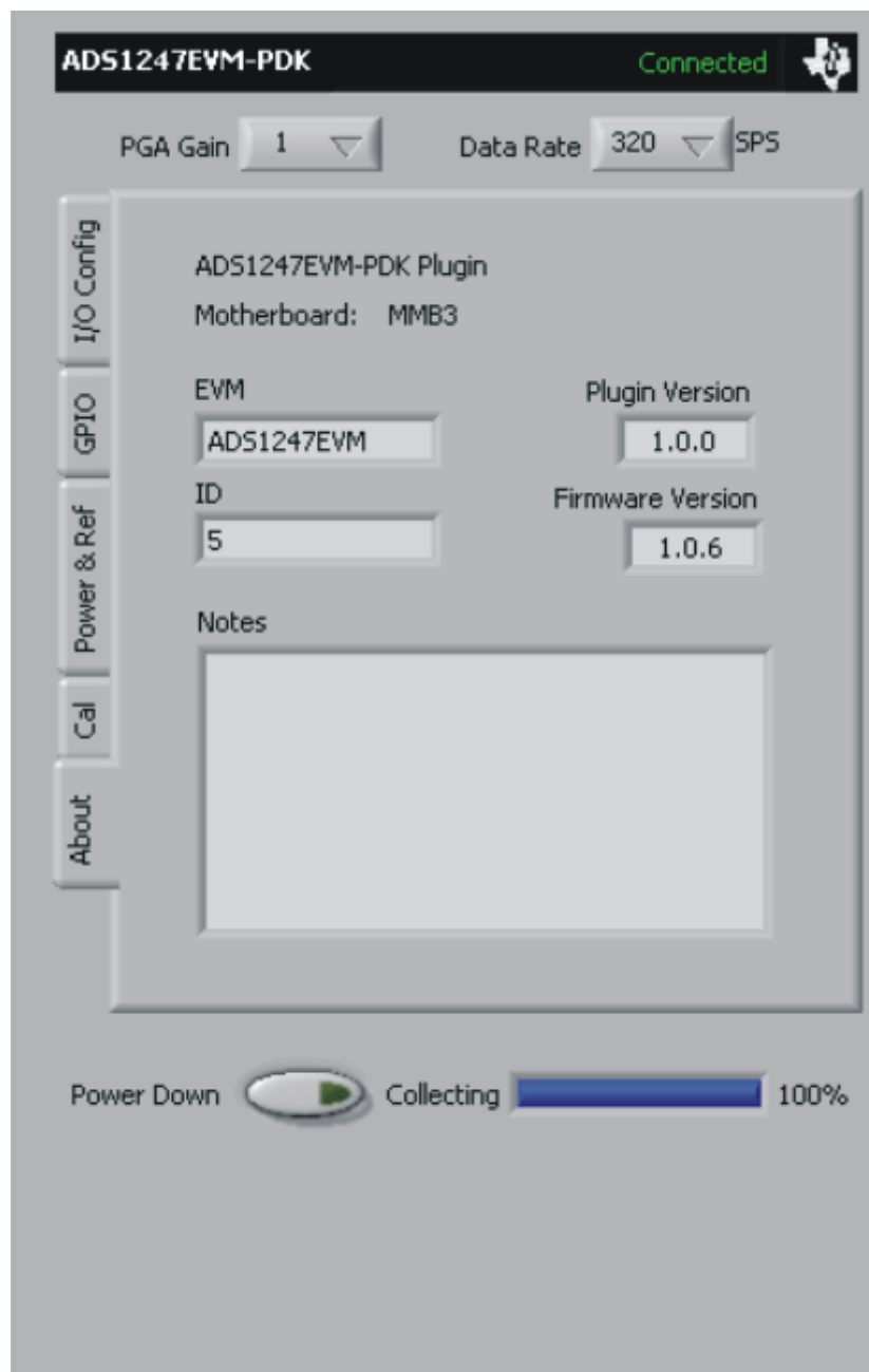
Figure 23. About Tab
