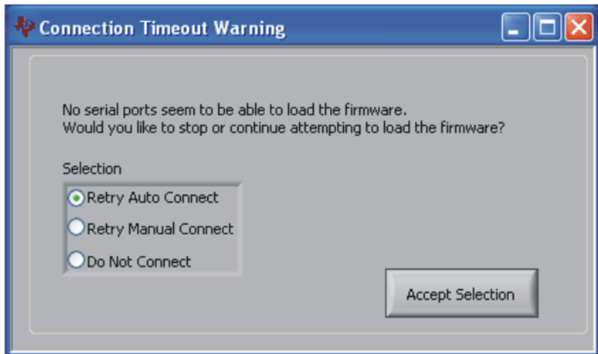
Figure 11. Connection Timeout
