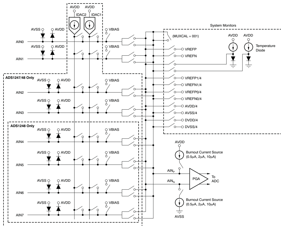
Figure 15. ADS1247 Multiplexer
