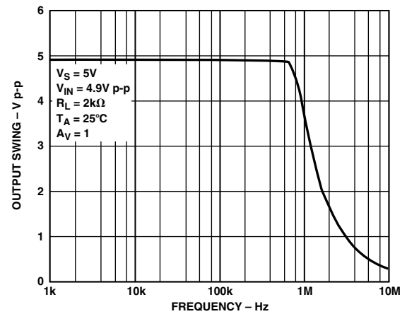
TPC 23. Closed-Loop Output Voltage Swing vs. Frequency
