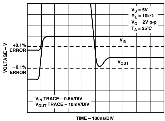
TPC 47. Settling Time
