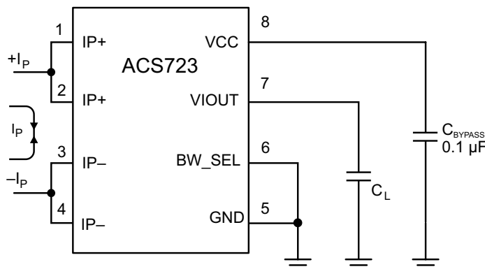
Typical Application
