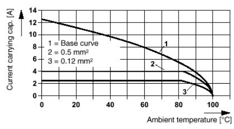
FK-MPT 0,5-ST-3,5 with PST 1,0
